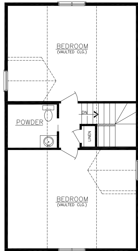
SECOND LEVEL AREA = 444 S.F. (USEABLE FLOOR AREA)
